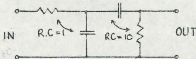
Fig. 4. Narrow band pass filter.
