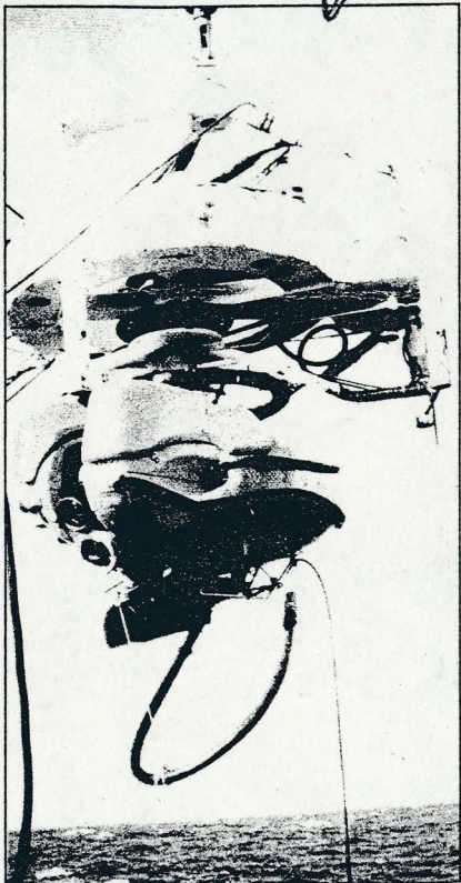
Fig. 9. Underwater flying observer (UFO) submersible rigged with thermoplastic hose, Scintillator, and radioactive pill in hose for calibration.
