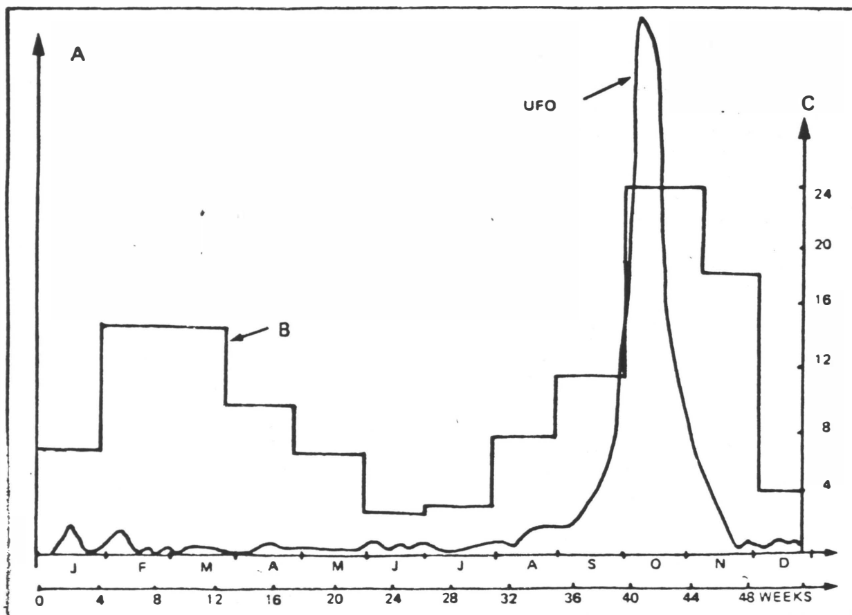
Fig. 3. To show the correlation between UFO observations in the earth's magnetic field during the year 1954 (635 French cases - Saunder's statistics). Key: A axis = Number of observations per week; B = Disturbances of the declination of the earth's magnetic field; C = number of disturbances of the magnetic declination per month
