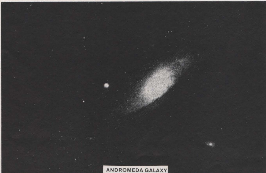
ANDROMEDA GALAXY
