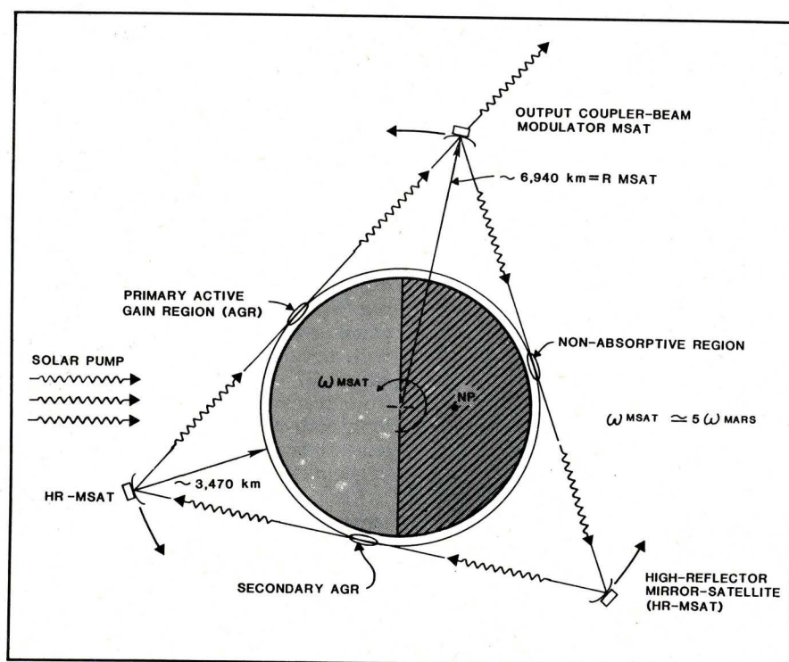
Figure 1. Schematic of proposed "Mars laser" to be used in the search for extra-terrestrial intelligence. The triangle formed by three mirrors created a ring laser with the Martian atmosphere as the lasing medium and the sun's energy as the pump.
