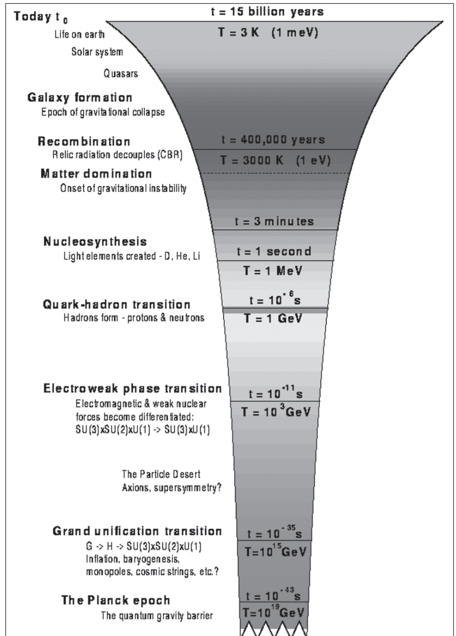
Standardmodellen for Universets utvikling.
